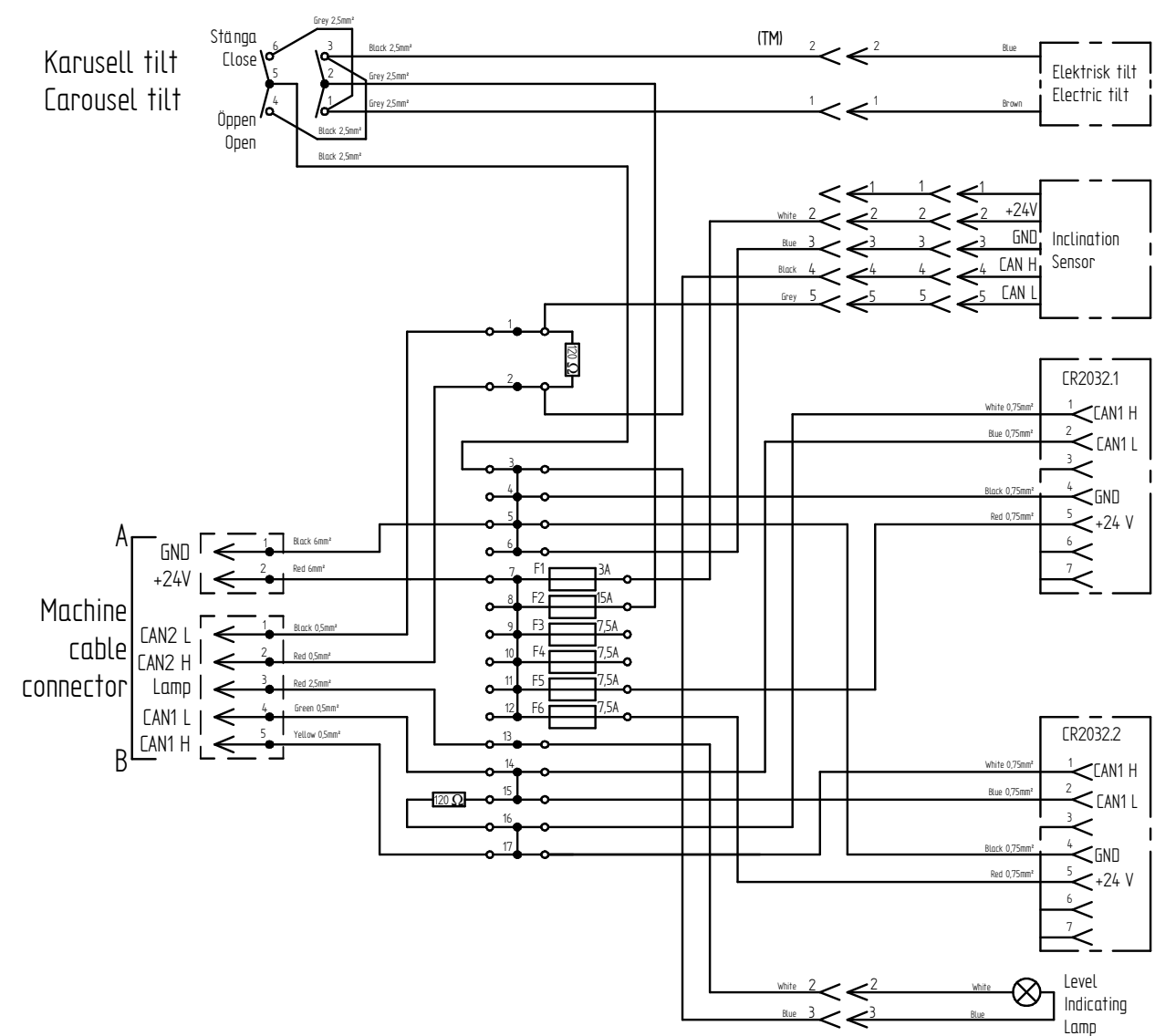
Junction Box in planter
